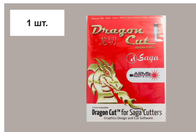
ПО DragonCut
